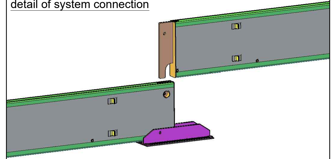
Wallstop AT Mobil 65-1 transition to steel elements
